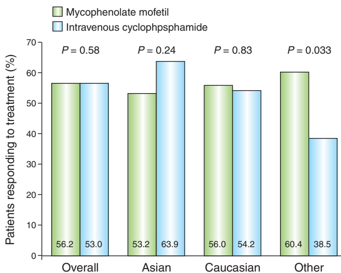
Figure 1. Rates of complete and partial remission in the Aspreva Lupus Management Study (ALMS) trial. After 6 months of therapy, induction therapy with either MMF or monthly intravenous cyclophosphamide pulses showed virtually identical rates of remission. In subgroup analyses by race, nonwhite and non-Asian subjects showed significantly higher rates of remission with MMF than cyclophosphamide. Reprinted from ref. 26.
